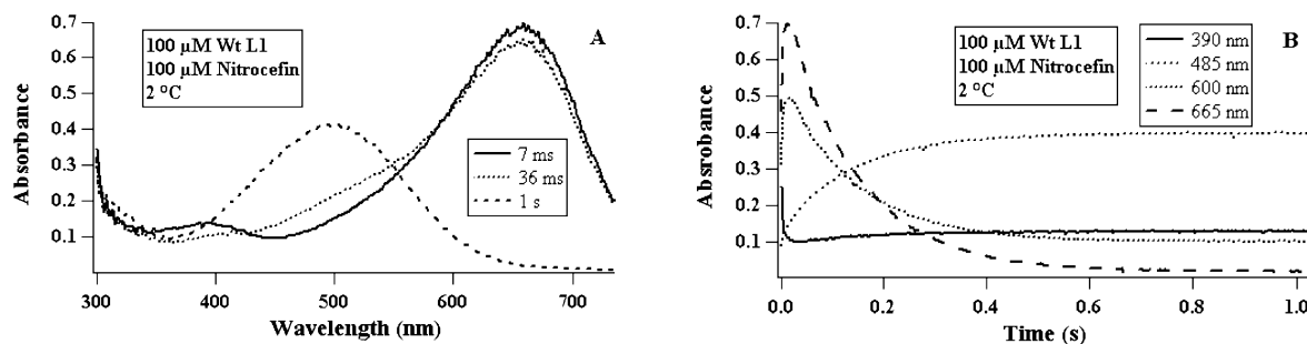
FIGURE 2: (A) Rapid-scanning electronic absorption spectra of the reaction of 100 \mu\text{M} wild-type L1 with 100 \mu\text{M} nitrocefin at 2 ^{\circ}\text{C} . (B) Single wavelength versus time plots of the reaction of 100 \mu\text{M} wild-type L1 with 100 \mu\text{M} nitrocefin at 2 ^{\circ}\text{C} . The buffer used in both reactions was 50 mM HEPES, pH 7.0.
