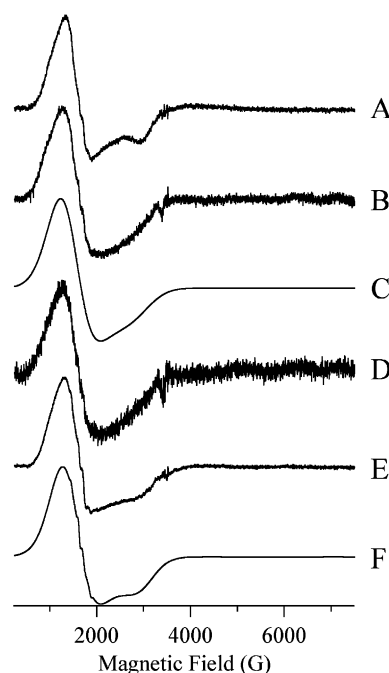
FIGURE 7: Trace A shows the resting EPR signal of Co(II)-L1. Traces B, D, and E show the EPR spectra of Co(II)-L1 upon reaction with penicillin G for 10 ms at 2 °C (B), 39 ms at 2 °C (D), and 60 s at 23 °C (E). Trace F shows the EPR spectrum of Co(II)-L1 upon incubation for 5 min at 23 °C with the L1-hydrolyzed product of penicillin G. Trace C is a computer simulation of (B) assuming S = 3/2 , D \gg \beta gBS (50 \text{cm}^{-1} ), M_S = |\pm 1/2\rangle , g_{xy} = 2.38 , g_z = 2.50 , and E/D = 0.005 . Trace F is a model for trace E and consists of (0.40 \times C) + (0.60 \times \text{trace B of Figure 4}) . Trace F also contains a 0.2% minor component due to Fe(III) with S = 5/2 , D = 20 \text{ cm}^{-1} , g_{\text{iso}} = 1.97 , and E/D = 0.244 . Experimental EPR spectra were recorded at 12 K with 1 mW microwave power at 9.63 GHz. 10 G (1 mT) field modulation at 100 kHz was employed.
