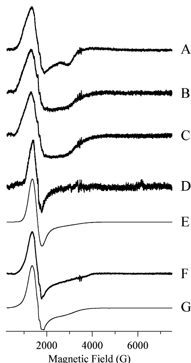
FIGURE 5: Trace A shows the resting EPR signal of Co(II)-L1. Traces B, C, and D show the EPR spectra of Co(II)-L1 upon reaction with cephalothin for 10 ms at 2 °C (B), 39 ms at 2 °C (C), and 60 s at 23 °C (D). Trace F shows the EPR spectrum of Co(II)-L1 upon incubation for 5 min at 23 °C with the L1-hydrolyzed product of cephalothin. Trace E is a computer simulation of (D) assuming S = 3/2 , D \gg \beta gBS ( 50 \text{ cm}^{-1} ), M_S = |\pm 1/2\rangle , g_{xy} = 2.28 , g_z = 2.35 , and E/D = 0.03 . Trace G also contains a 0.2% minor component due to Fe(III) with S = 5/2 , D = 20 \text{ cm}^{-1} , g_{\text{iso}} = 1.97 , and E/D = 0.244 . Experimental EPR spectra were recorded at 12 K with 1 mW microwave power at 9.63 GHz. 10 G (1 mT) field modulation at 100 kHz was employed.
