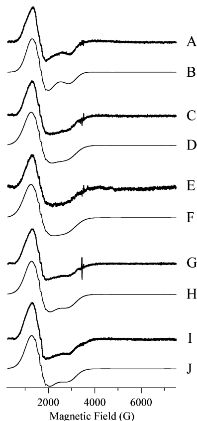
FIGURE 4: Trace A shows the resting EPR signal of Co(II)-L1. Traces C, E, and G show the EPR spectra of Co(II)-L1 upon reaction with nitrocefins for 10 ms at 2 ^{\circ}\text{C} (C), 39 ms at 2 ^{\circ}\text{C} (E), and 30 s at 23 ^{\circ}\text{C} (G). Trace I shows the EPR spectrum of Co(II)-L1 upon incubation for 5 min at 23 ^{\circ}\text{C} with the L1-hydrolyzed product of nitrocefins. Trace B is a computer simulation of (A) assuming S = 3/2 , D \gg \beta gBS ( 50 \text{ cm}^{-1} ), M_S = |\pm 1/2\rangle , g_{xy} = 2.32 , g_z = 2.35 , and E/D = 0.03 . Trace F is a computer simulation of (E) assuming S = 3/2 , D \gg \beta gBS ( 50 \text{ cm}^{-1} ), M_S = |\pm 1/2\rangle , g_{xy} = 2.31 , g_z = 2.42 , and E/D = 0.03 . Traces B and F also contain a 0.2% minor component due to Fe(III) with S = 5/2 , D = 20 \text{ cm}^{-1} , g_{iso} = 1.97 , and E/D = 0.244 . Traces D, H, and J are models for traces C, G, and I, respectively, and consist of (0.15 \times B) + (0.85 \times F) (D), (0.50 \times B) + (0.50 \times F) (H), and (0.52 \times B) + (0.48 \times F) (J). Experimental EPR spectra were recorded at 12 K with 1 mW microwave power at 9.63 GHz. 10 G (1 mT) field modulation at 100 kHz was employed.
