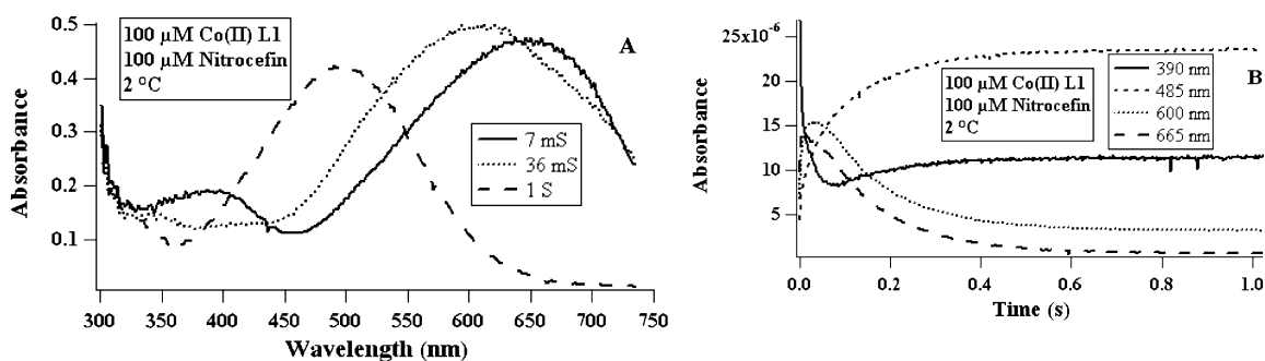
FIGURE 3: (A) Rapid-scanning electronic absorption spectra of the reaction of 100 \mu\text{M} Co(II)-substituted L1 with 100 \mu\text{M} nitrocefins at 2 ^{\circ}\text{C} . (B) Single wavelength versus time plots of the reaction of 100 \mu\text{M} Co(II)-substituted L1 with 100 \mu\text{M} nitrocefins at 2 ^{\circ}\text{C} . The buffer used in both reactions was 50 mM HEPES, pH 7.0.
